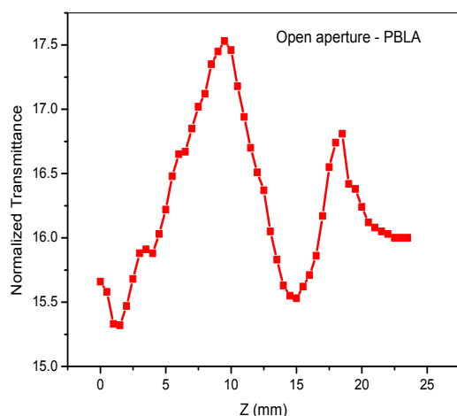
Fig.7: Open aperture z-scan curve of PBLA crystal
